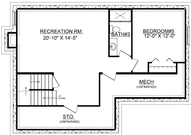
Basement 677 sq.ft.
